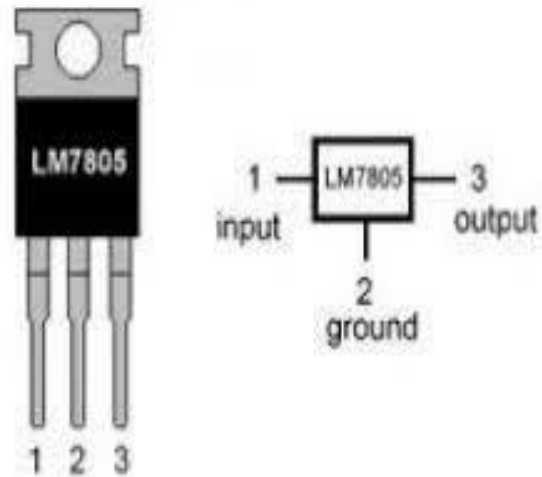
LM7805 PINOUT DIAGRAM
